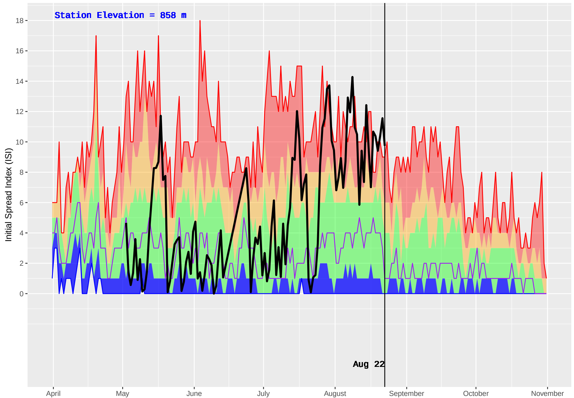
BEDNESTI (175) : Historical (1993–2016) and Current (2018) Daily Initial Spread Index (ISI)
